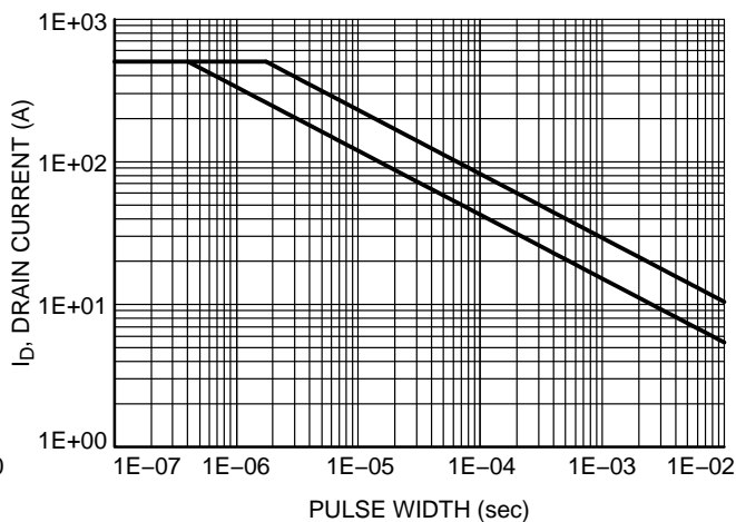
Figure 15. Avalanche Characteristics
